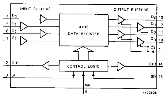
Fig. 4 Functional diagram.
