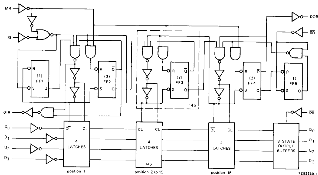
Fig. 5 Logic diagram.
