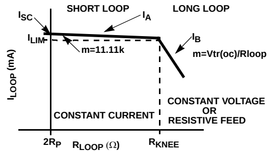
FIGURE 3. I_{\text{LOOP}} vs. R_{\text{LOOP}} LOAD CHARACTERISTIC
