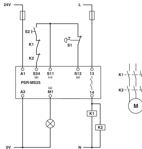
Figure 14 Emergency stop monitoring/manual, monitored start
