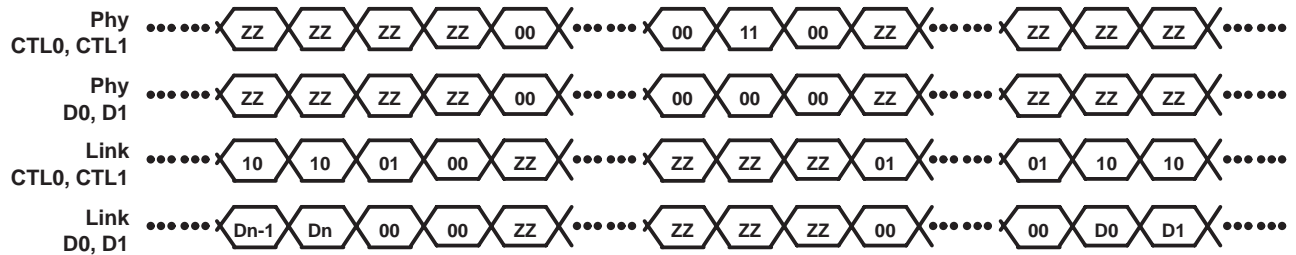
Figure 6. Transmit Timing
