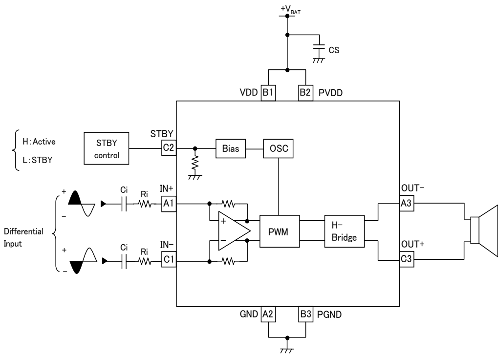
Figure.36 Differential input for mobile phone
