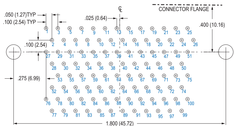
100 PIN M83513/12-H
