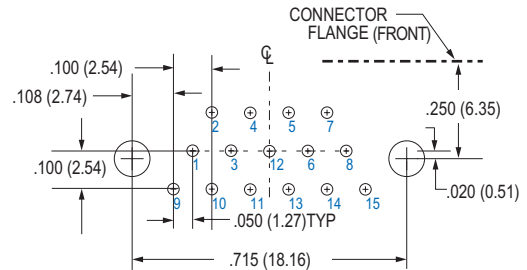
15 PIN M83513/10-B
