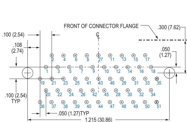
51 PIN M83513/11-G
