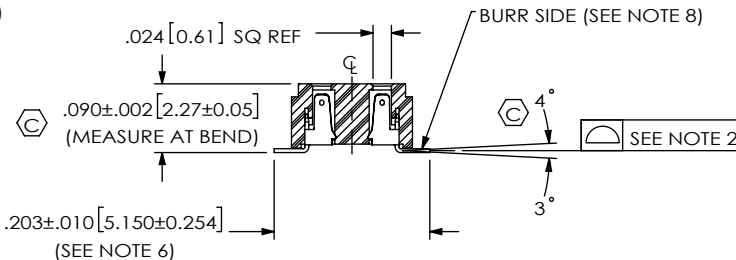
SECTION "A"-"A" SCALE 4:1
