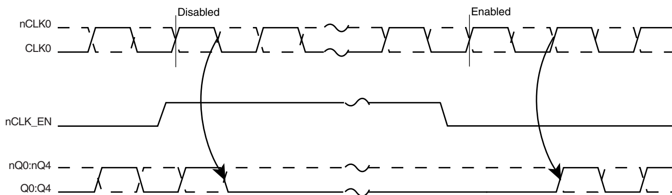
FIGURE 1. nCLK_ENTIMING DIAGRAM
