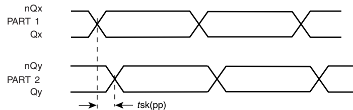
PART-TO-PART SKEW
