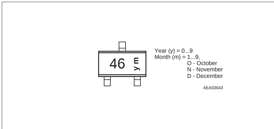
Figure 4 Marking TLE4946K
