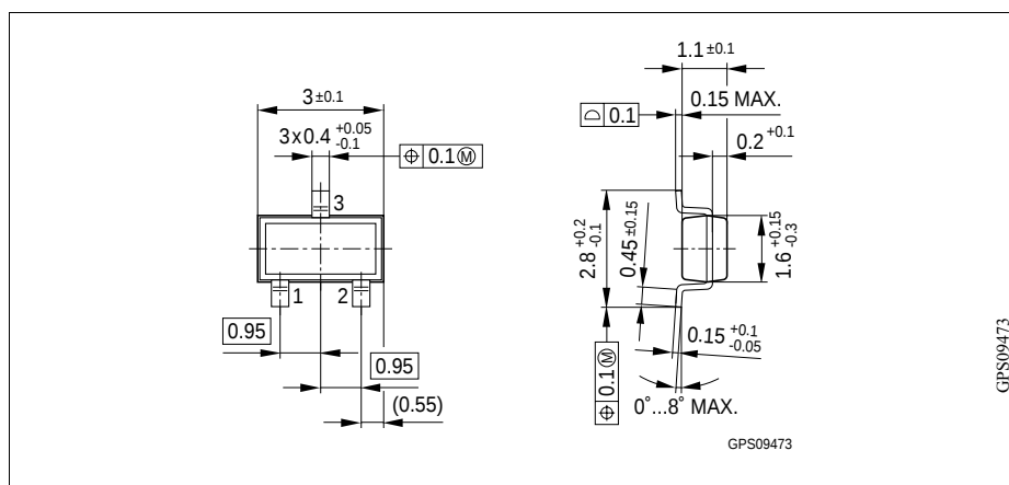
Figure 6 SC59
