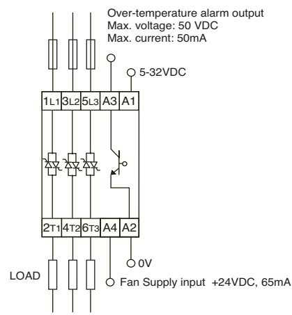
DC Control Input + Fan + over-temperature protection Example: RJ3A60D32EP
