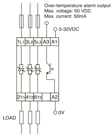
DC Control Input + over-temperature protection Example: RJ3A60D20EP
