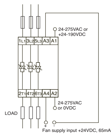
AC Control Input + fan + over-temperature protection Example: RJ3A22A32EP
