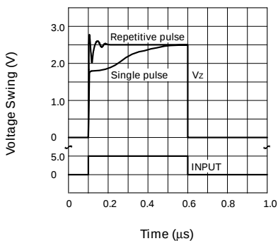
Pulse Response
