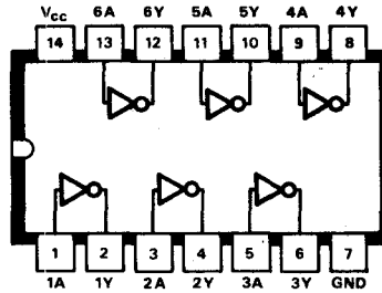
B6 SN7405N/AN SN74H05N/SN74S05N Hex Inverter with open collector output
