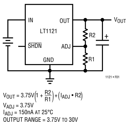
Figure 1. Adjustable Operation
