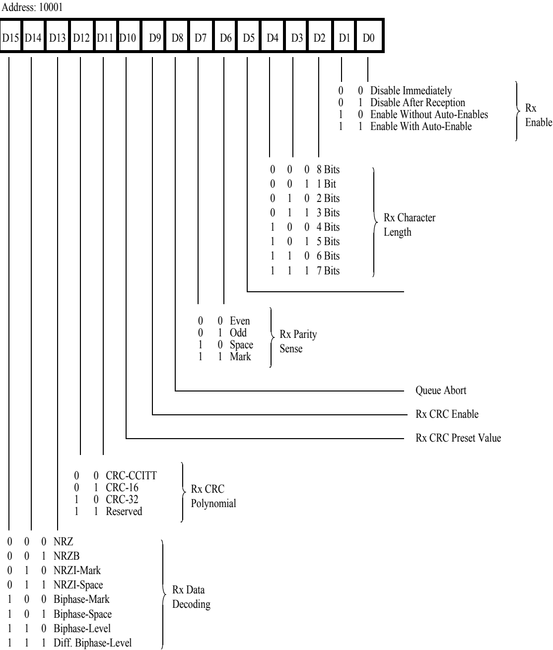
Figure 59. Receive Mode Register
