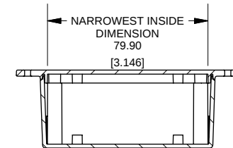
SECTION C-C SCALE 3 / 8
