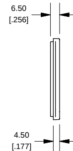
SIDE VIEW OF LID
