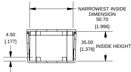
SECTION B-B SCALE 3 / 8
