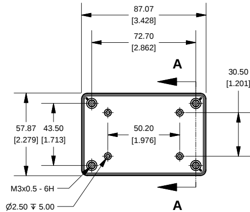
TOP VIEW OF BOX
