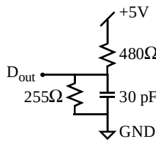
Figure B: Output Load AS7C256-09
