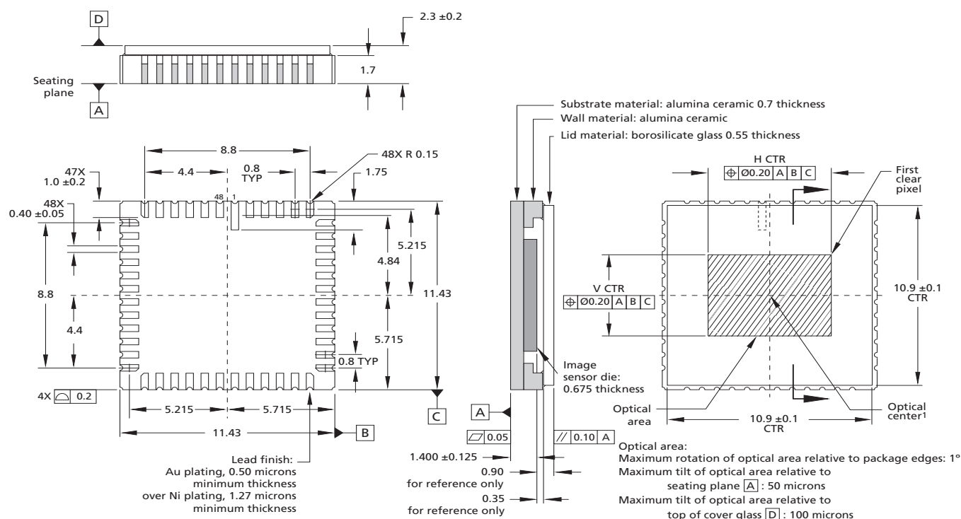
Figure 10: 48-Pin CLCC Package Outline
