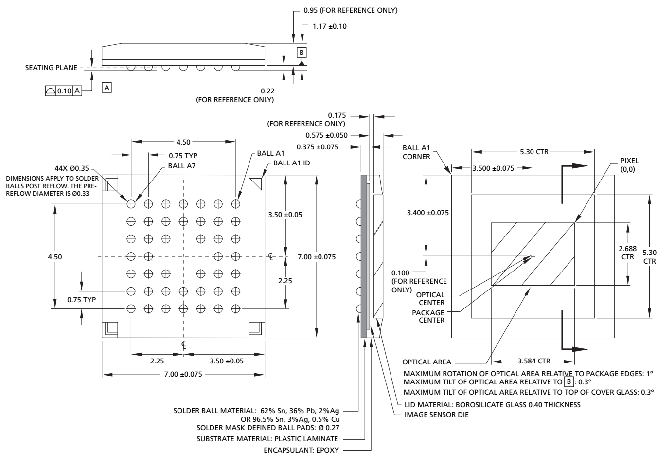
Figure 9: 44-Ball iCSP Package Outline
