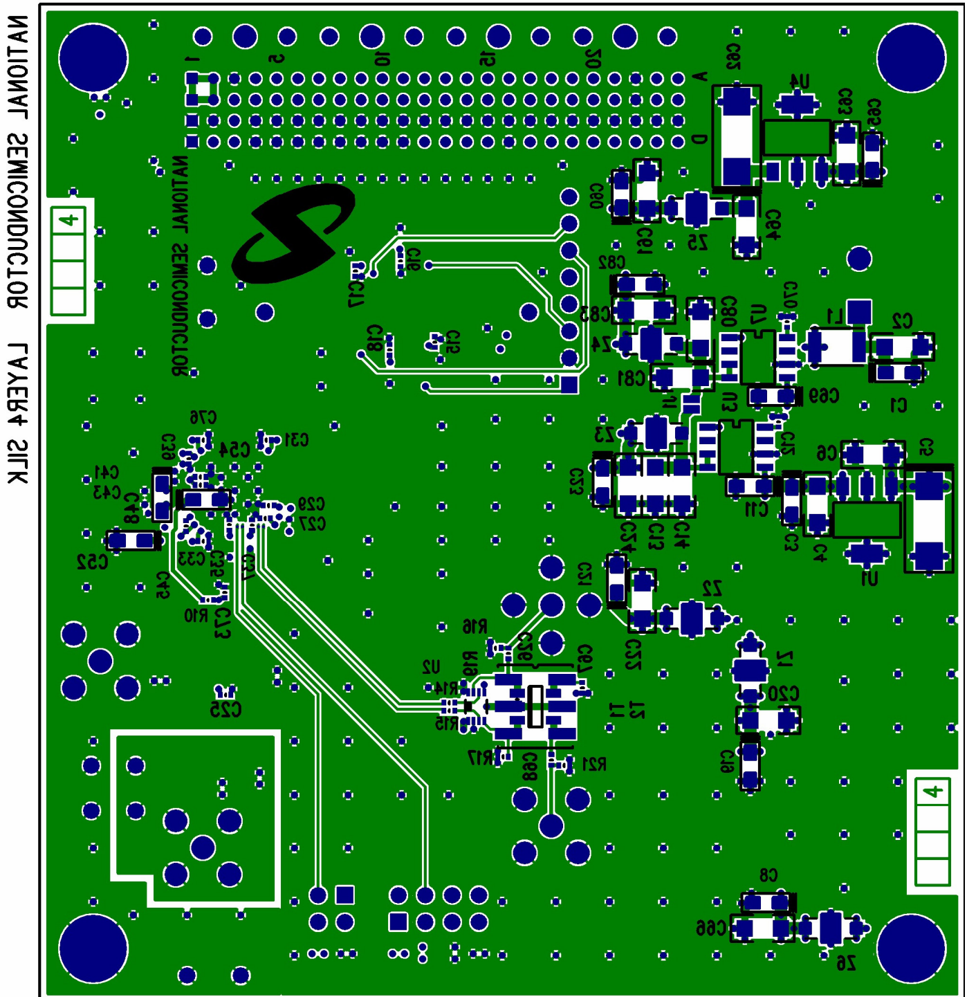
Figure 9. Layer 4 - Signal
