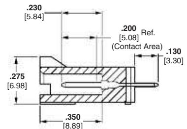
Section X-X
