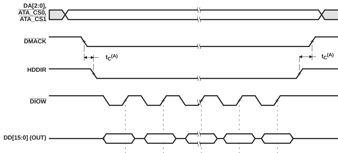
Figure 7-79. ATA HDDIR Multiword DMA Write Transfer Timing
