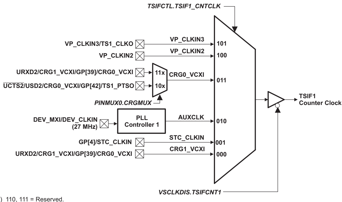
Figure 7-45. TSIF1 Counter Clock Selection
