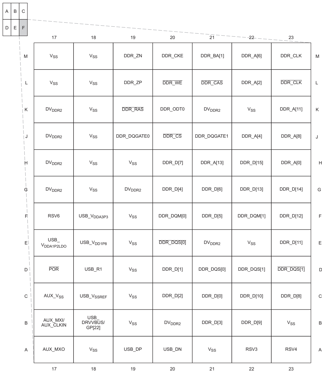
Figure 3-7. Pin Map [Section F]
