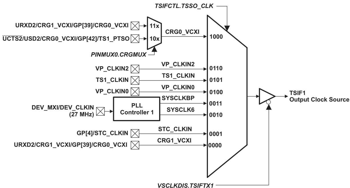
Figure 7-44. TSIF1 Output Clock Source Selection
