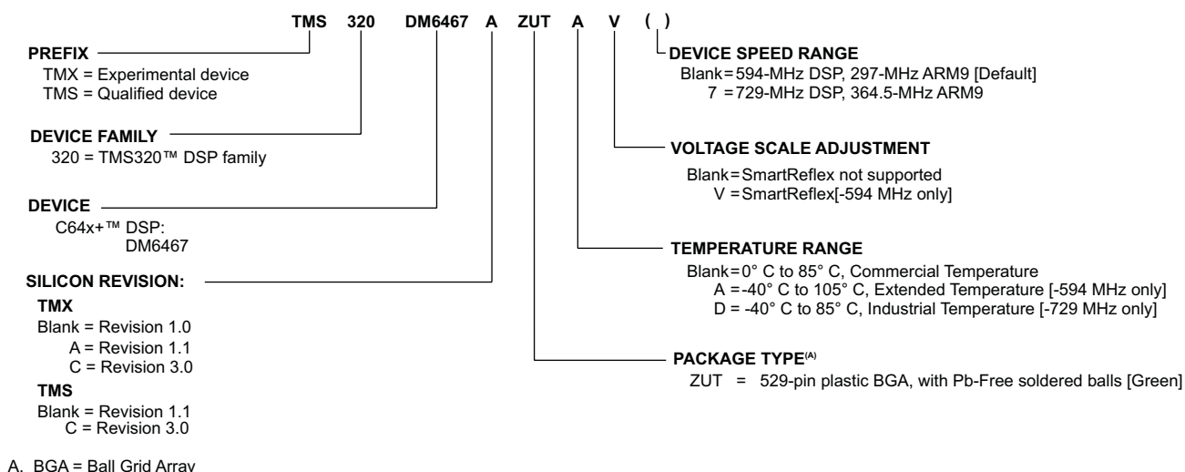
Figure 3-8. Device Nomenclature
