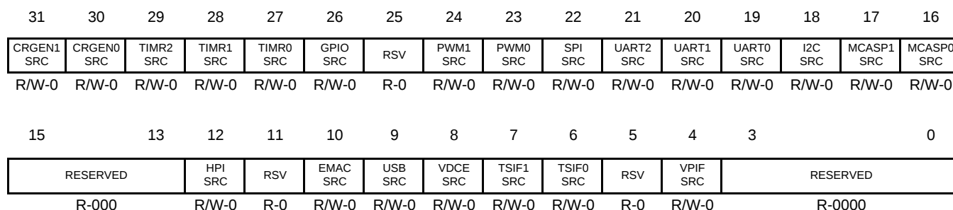
Figure 4-26. SUSPSRC Register
