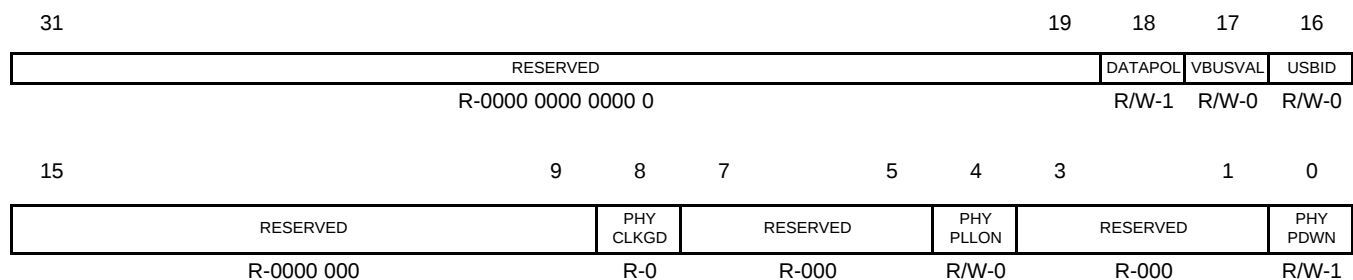
Figure 4-15. USBCTL Register [0x01C4 0034]
