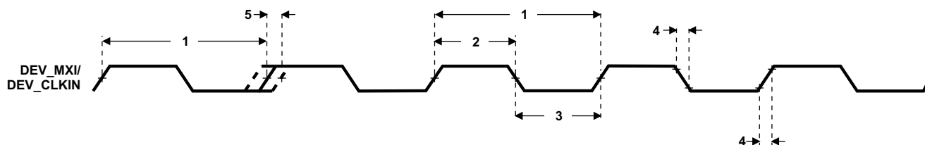
Figure 7-16. DEV_MXI/DEV_CLKIN Timing
