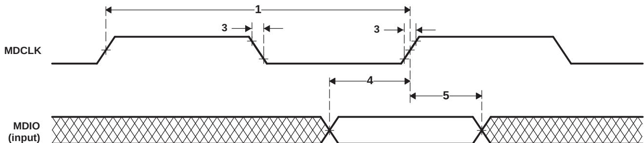
Figure 7-57. MDIO Input Timing
