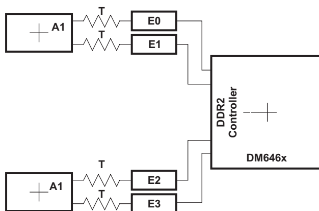
Figure 7-33. DQS and DQ Routing and Topology
