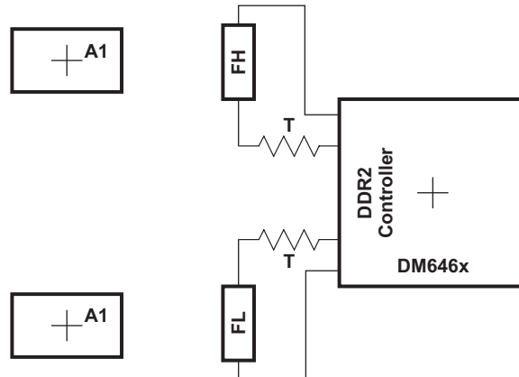
Figure 7-34. DQGATE Routing
