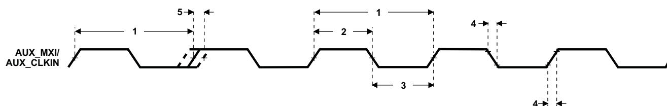
Figure 7-17. AUX_MXI/AUX_CLKIN Timing
