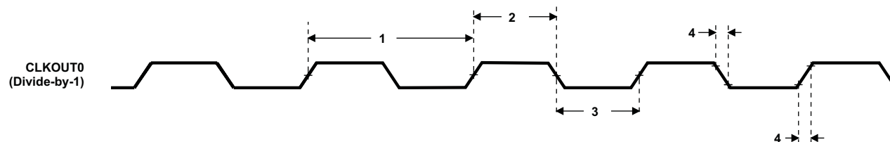
Figure 7-18. CLKOUT0 Timing
