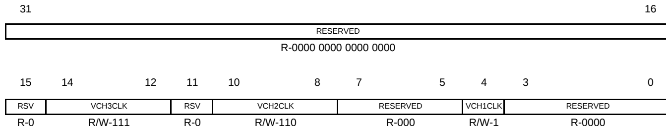
Figure 4-2. VIDCLKCTL Register [0x01C4 0038]
