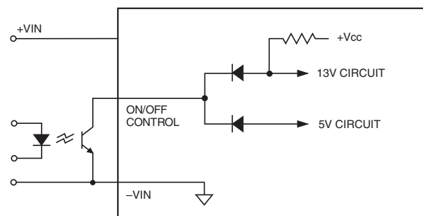
Figure 4. Driving the Negative Logic On/Off Control Pin (simplified circuit)
