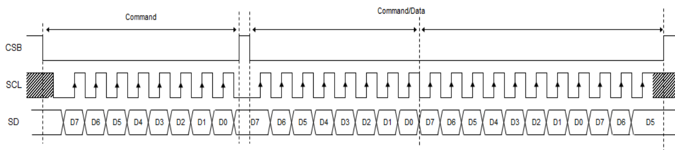
Figure 7. 3-SPI Data Transfer Format
