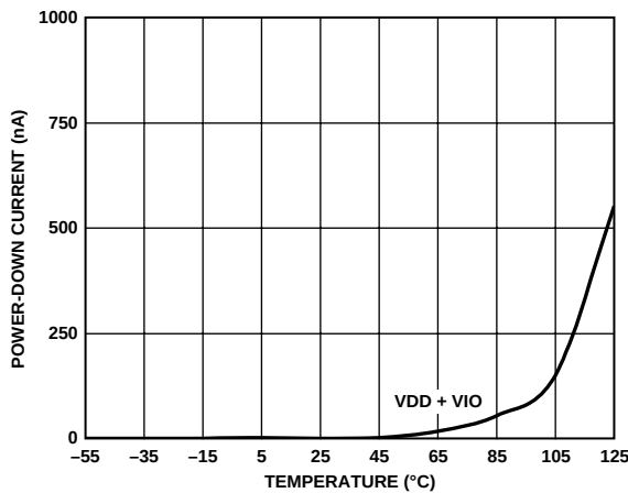
Figure 20. Power-Down Currents vs. Temperature
