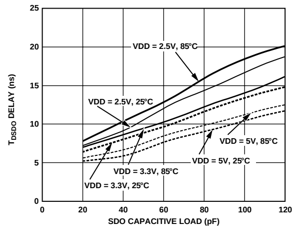
Figure 23. t_{DSO} vs. Capacitance Load and Supply
