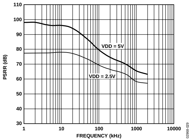
Figure 30. PSRR vs. Frequency
