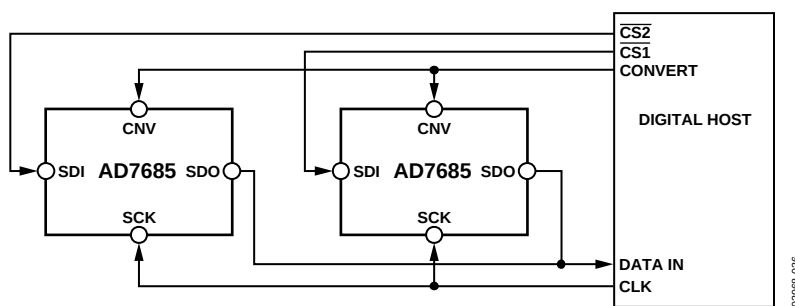
Figure 37. \overline{\text{CS}} Mode 4-Wire, No \text{BUSY} Indicator Connection Diagram
