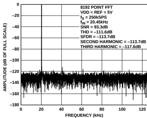
Figure 8. FFT Plot
