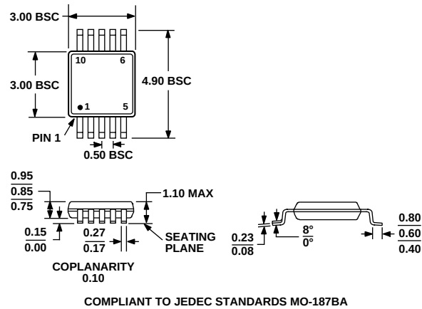
Figure 48. 10-Lead Micro Small Outline Package [MSOP] (RM-10) Dimensions shown in millimeters
