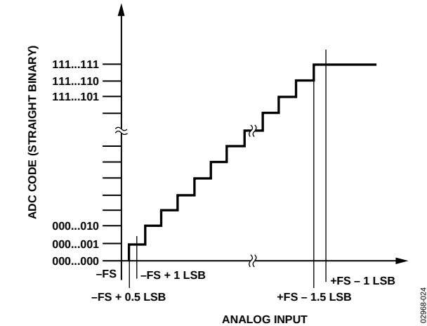
Figure 25. ADC Ideal Transfer Function
