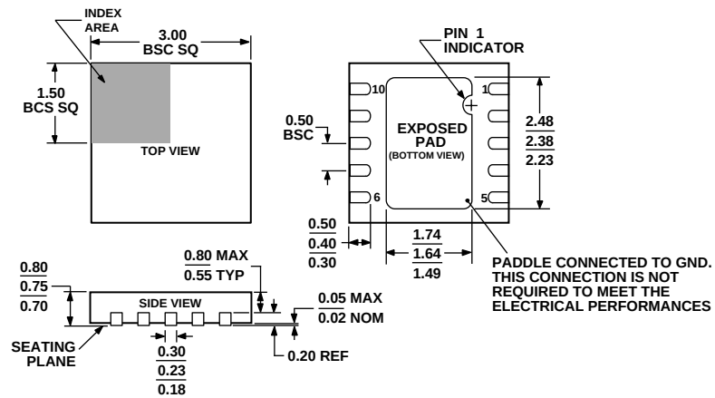
Figure 49. 10-Terminal Quad Flat No Lead Package [QFN 1 (LFCSP)] 3 mm × 3 mm Body (CP-10-9) Dimensions shown in millimeters
