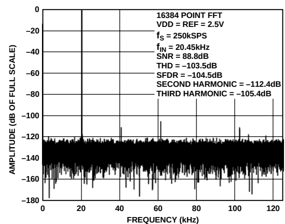
Figure 11. FFT Plot
