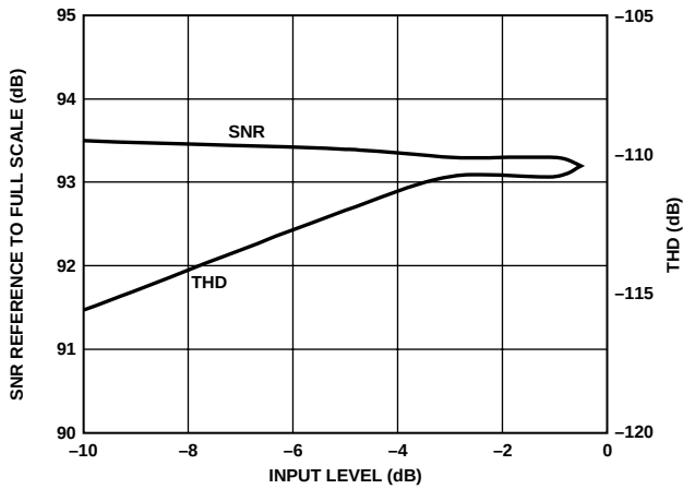
Figure 18. SNR and THD vs. Input Level
