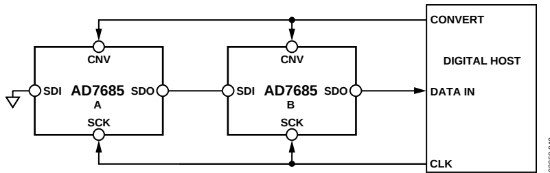
Figure 41. Chain Mode Connection Diagram
