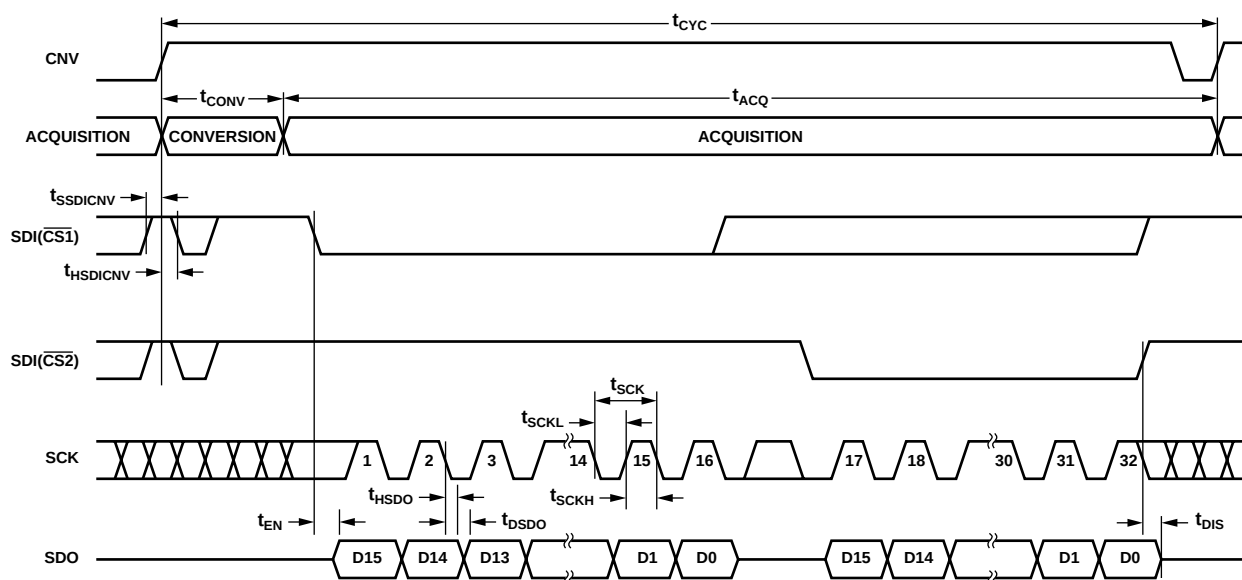
Figure 38. \overline{\text{CS}} Mode 4-Wire, No \text{BUSY} Indicator Serial Interface Timing
