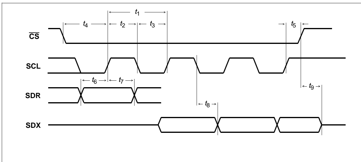
Figure 72 SCI Interface
