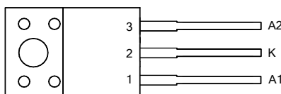
TO-220F-3 (Option 1)
