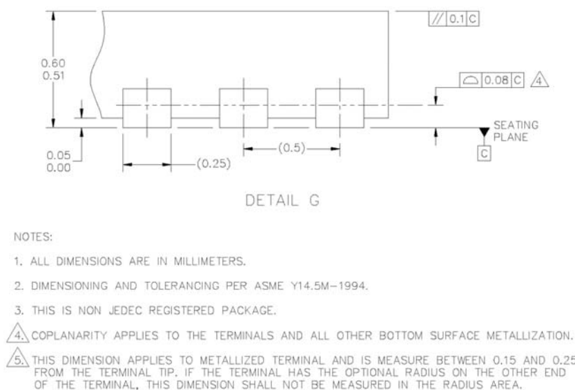
Figure 23. Package Details
