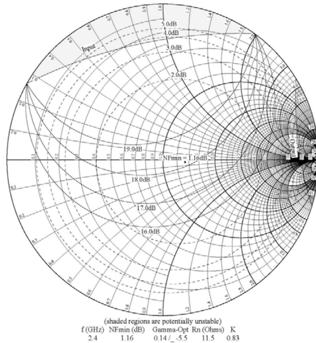
Figure 21. Constant Noise Figure and Gain Circles, 2400 MHz, R_{bias}=1.5\text{ k}\Omega
