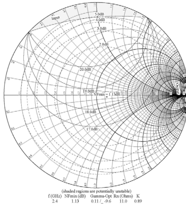
Figure 20. Constant Noise Figure and Gain Circles, 2400 MHz, R_{bias}=1.2\text{ k}\Omega
