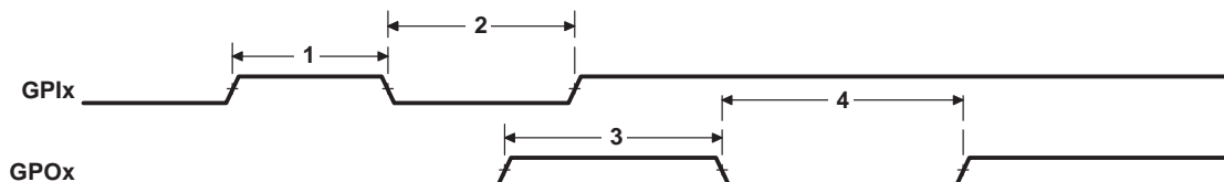
Figure 7–45. GPIO Port Timing
