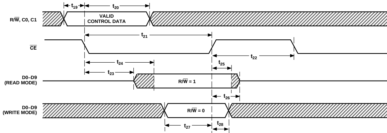
Figure 14. Microprocessor Port (MPU) Interface Timing
