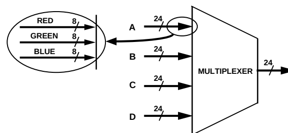
Figure 15. Multiplexed Color Inputs for the ADV7160/ADV7162
