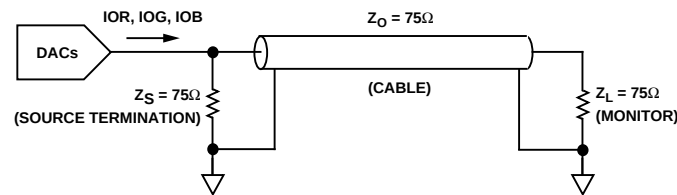
Figure 46. DAC Output Termination (Doubly Terminated 75 \Omega Load)
