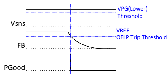
Figure 21: Timing Diagram for Open Feedback Line Protection (OFLP)
