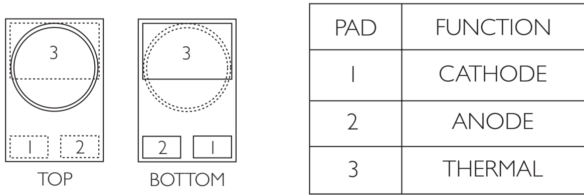
Figure 2. Pad configuration.
