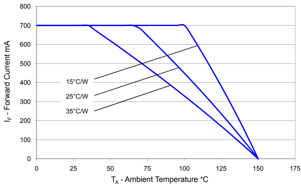
Figure 18. Maximum forward current vs. ambient temperature, based on T JMAX = 150°C.
