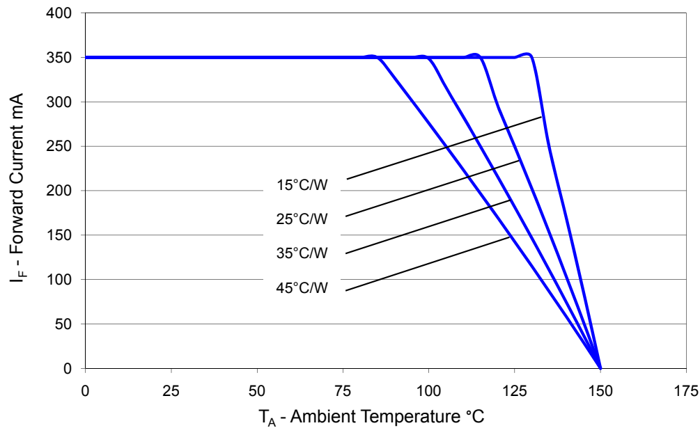
Figure 17. Maximum forward current vs. ambient temperature, based on T JMAX = 150°C.
