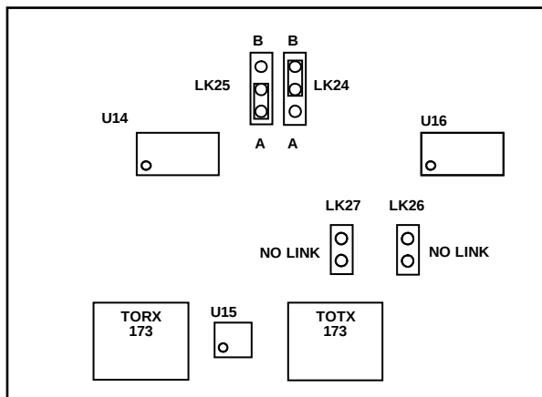
Figure 3. Link Positions
