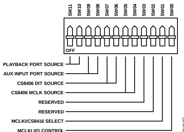
Figure 2. Switches Configuration
