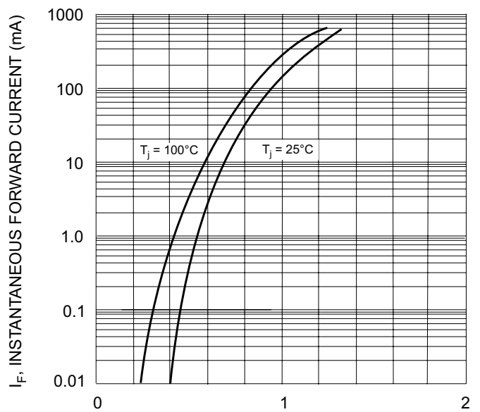
Fig. 2 Forward Characteristics 1N914B
