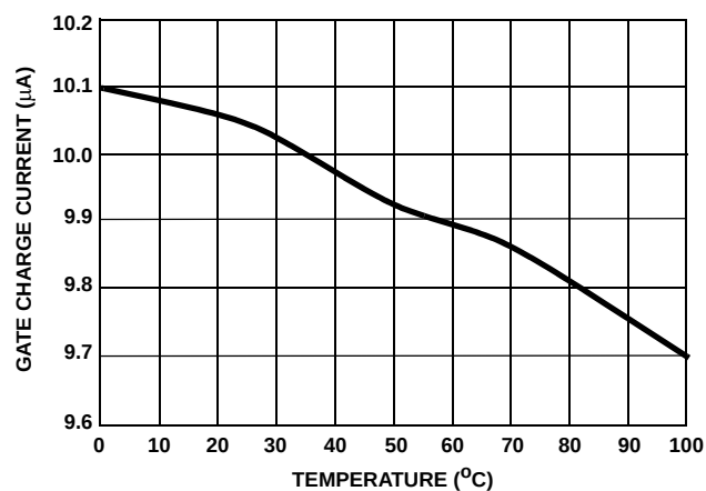
FIGURE 10. GATE CHARGE CURRENT
