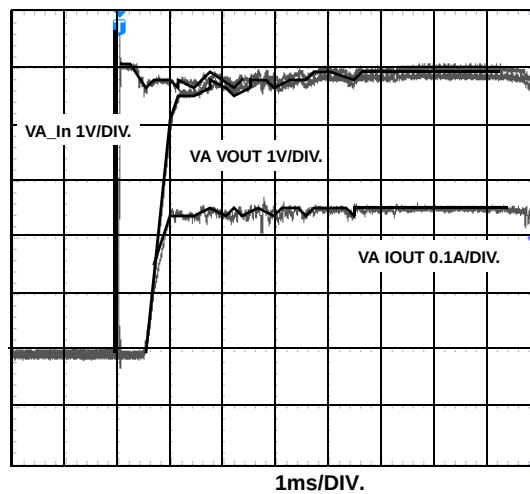
FIGURE 18. VA HOT SWAP TURN-ON
