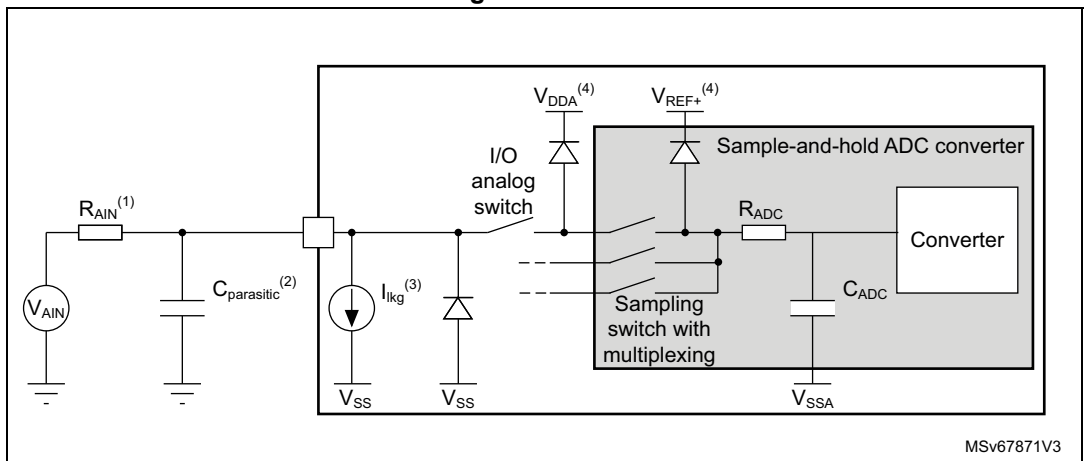
analog switch function
