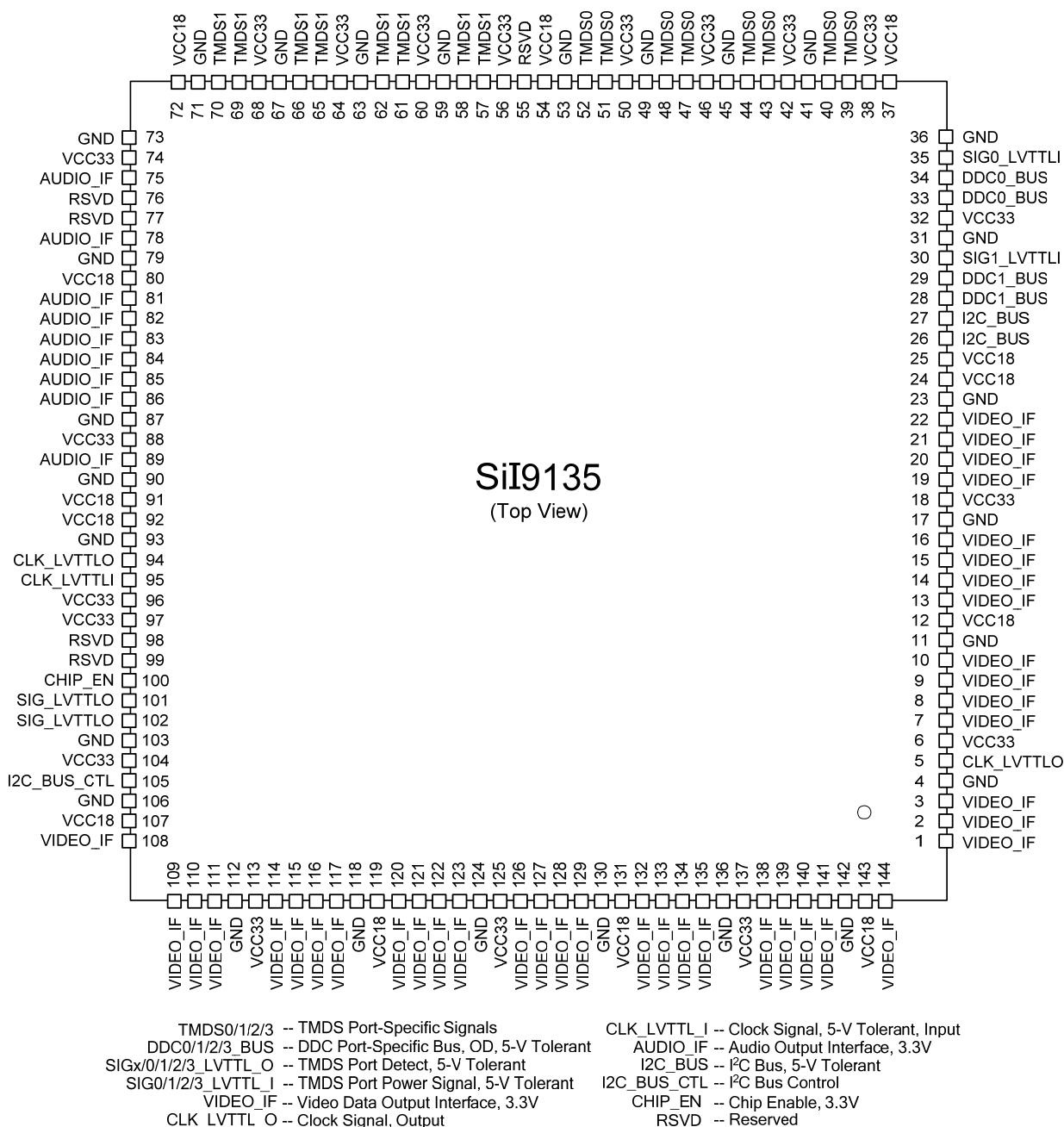
Figure 2. Pin Diagram
