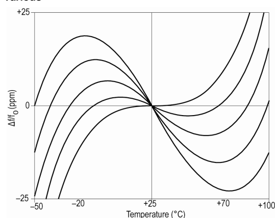
Typical Frequency vs Temperature Curves for various
