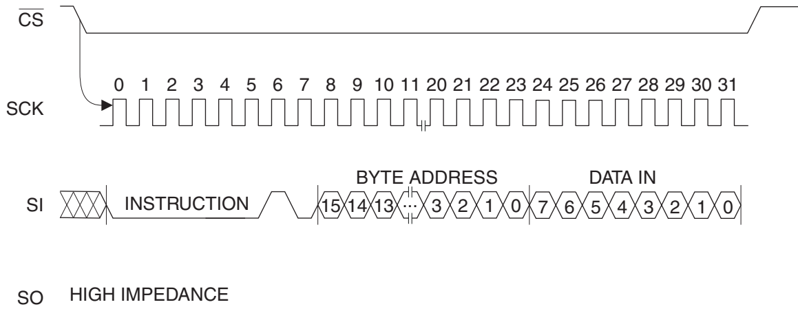
Figure 3-7. WRITE Timing
