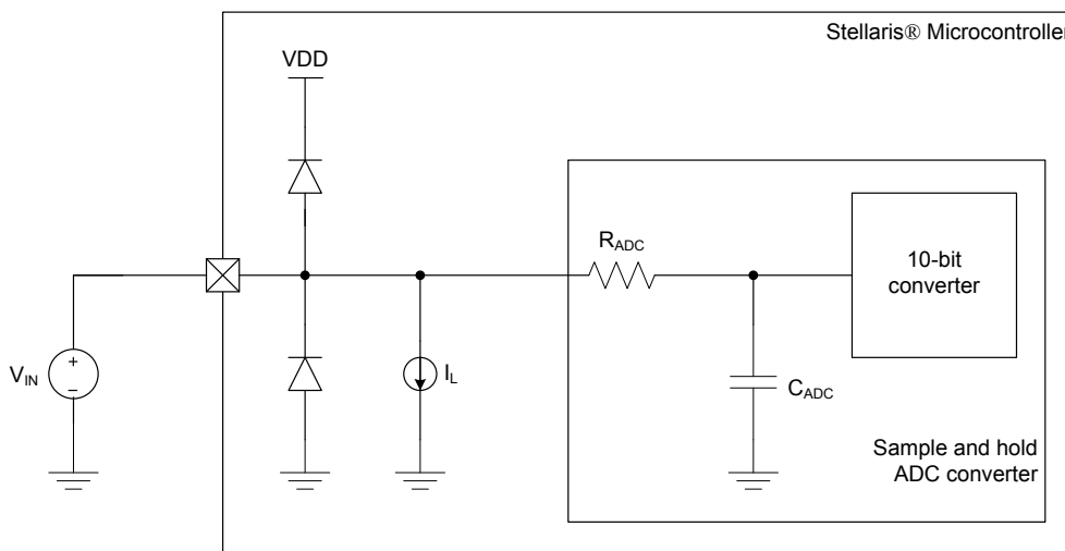
Figure 19-11. ADC Input Equivalency Diagram
