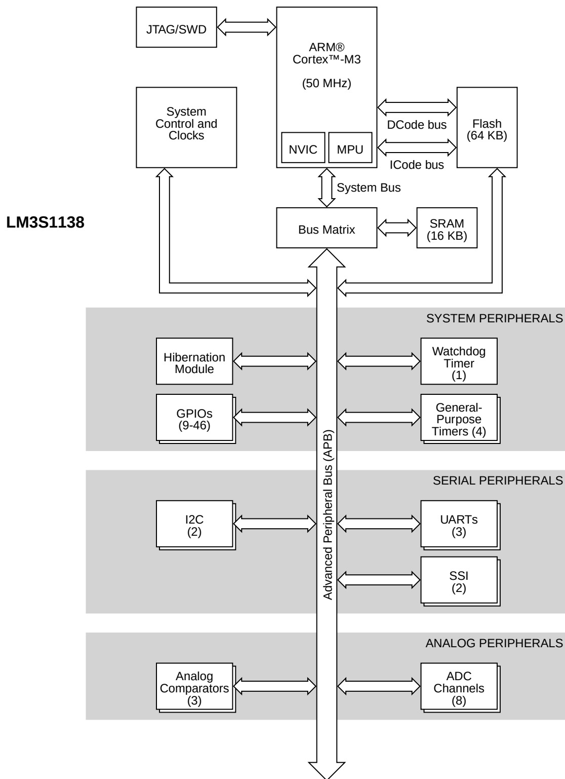
Figure 1-1. Stellaris LM3S1138 Microcontroller High-Level Block Diagram
