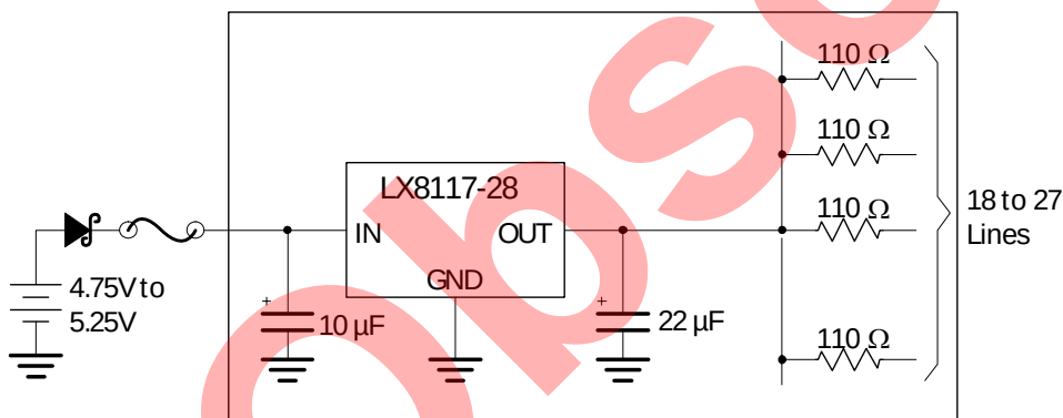
ACTIVE TERMINATOR FOR SCSI-2 BUS
