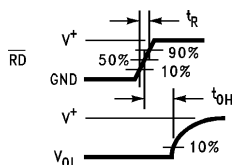
Figure 41. TRI-STATE Test Circuits and Waveforms
