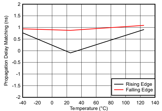
Figure 6-17. Propagation Delay Matching, Rising and Falling Edge
