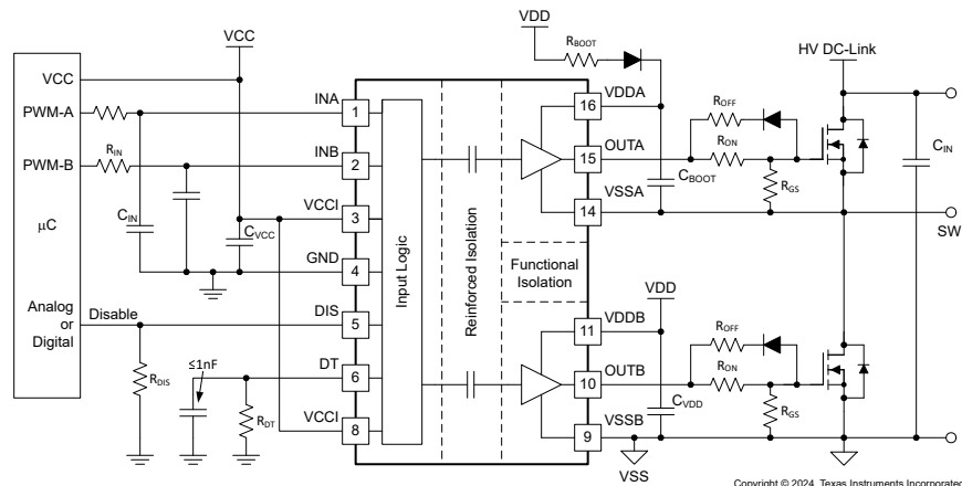
Typical Application
