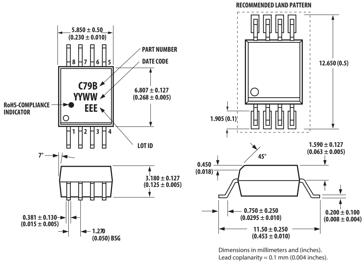
Figure 2. SS0-8 package.
