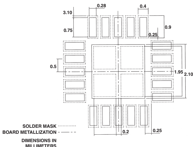
Figure 3. Suggested LFCSP 4 mm \times 4 mm 20-Lead Land Pattern
