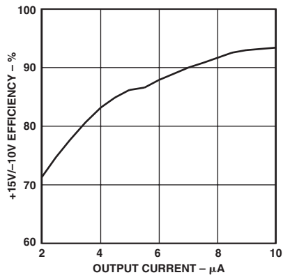
TPC 5. +15V/-10V Efficiency vs. Output Current in Blanking Mode, V_{CC} = 3\text{ V}
