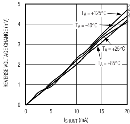
LM4040-2.5V REVERSE VOLTAGE vs. I_{SHUNT}
