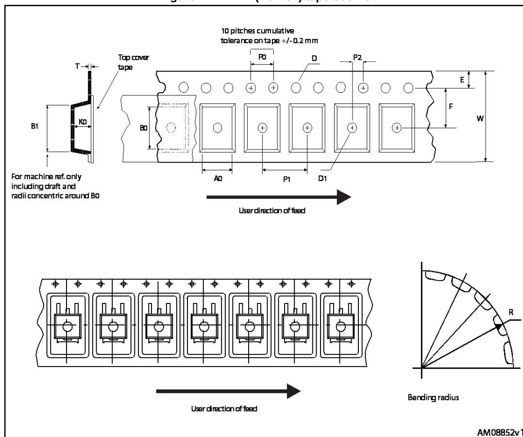
Figure 27: DPAK (TO-252) tape outline
