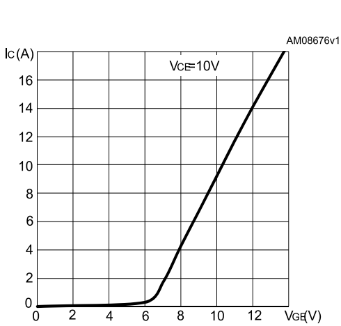
Figure 4: Transfer characteristics
