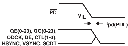
Figure 7. Delay From \overline{\text{PD}} Low to Hi-Z Outputs
