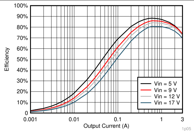
Figure 7-10. V_{OUT} = 1.05\text{-V} Efficiency, L = 1.5\text{ }\mu\text{H}
