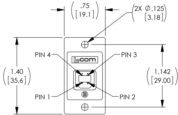
USB TYPE "B" JACK "J1"
