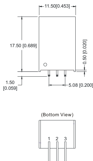
V78XX-2000R
