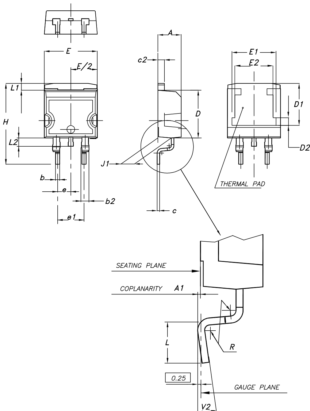
Figure 38. D 2 PAK (TO-263) type A package outline
